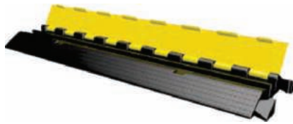
DCPR0002 2 Channel Flexible Cable Protector Size : L980 x W240 x H44mm Hole Size : L30 x H30mm
