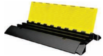
DCPR0003 3 Channel Flexible Cable Protector Size : L900 x W500 x H75mm Hole Size : L63 x H53mm
